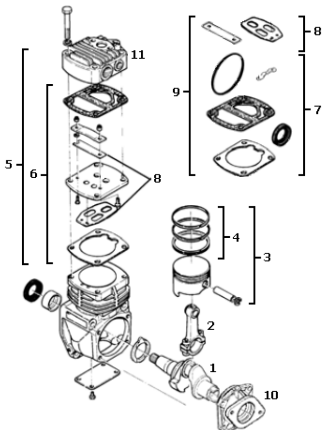
Compressore con attacco pompa trasversale. Compressor with diagonal pump coupling.
