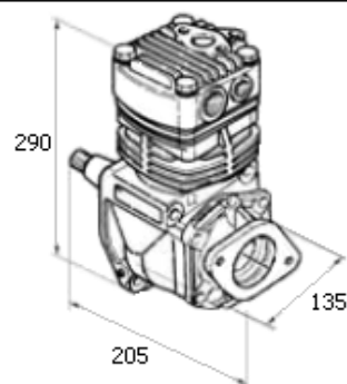
Compressore con attacco pompa trasversale. Compressor with diagonal pump coupling.
