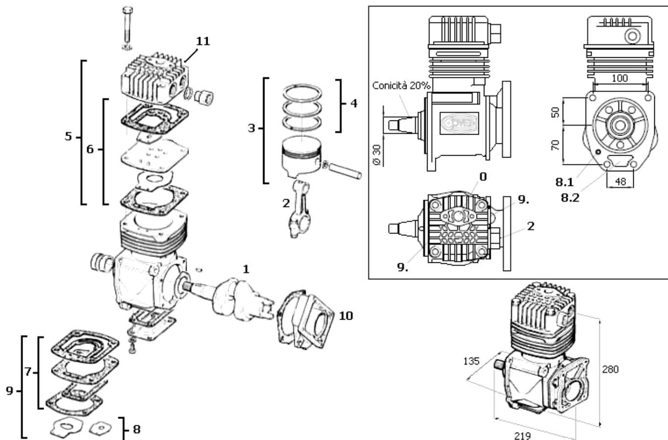
Compressore con attacco pompa trasversale. Compressor with diagonal pump coupling.
